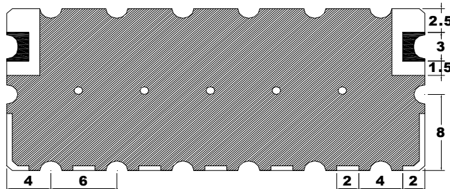
BOTTOM VIEW
